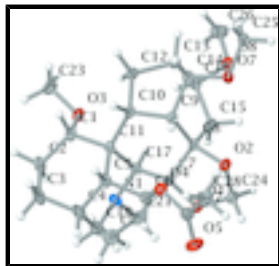
Fig. 1. The molecular structure of the title compound with the atom numbering, showing displacement ellipsoids at the 30% probability level.
